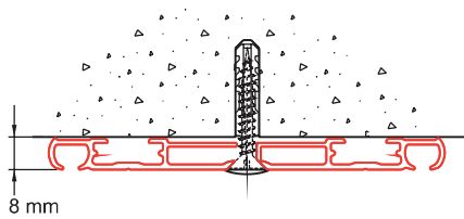
ceiling mounting of pre-drilled 2905 with 2914-WD screw with white cover cap
