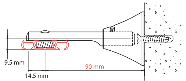
wall mounting 2901 with wall bracket 2917-09
